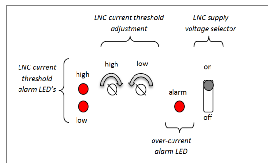
LNC input connection status and configuration
